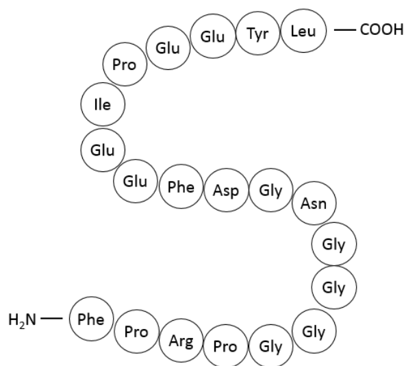
Figure 1: Structural Formula of Bivalirudin
