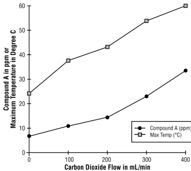
Figure 2: Carbon Dioxide Flow Versus Compound A and Maximum Temperature
